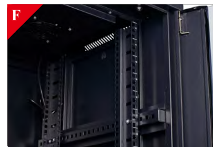
Front and rear sets of vertical rails adjust in quarter inch increments. Simply unscrew the rails, adjust them to the required depth and re-fasten.
