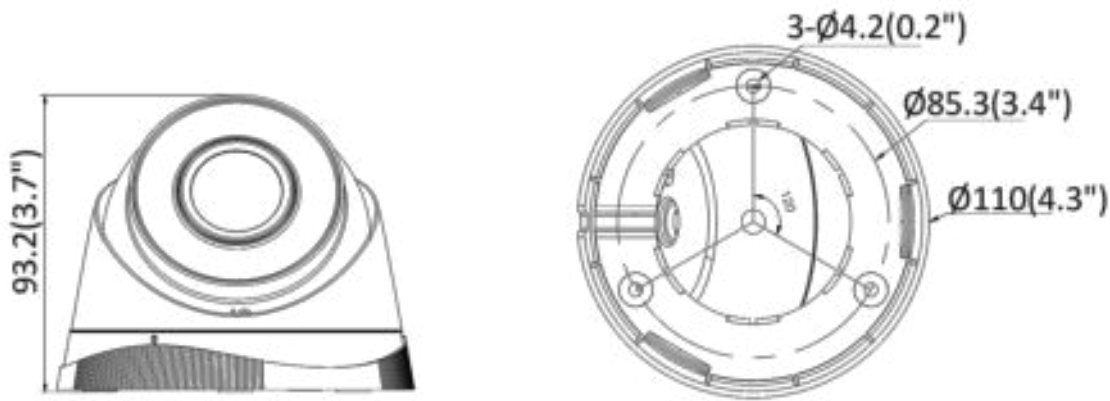
Unit: mm(inch)
